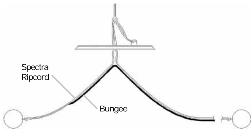
FIGURE 2 RIPCORDERDETAIL (Housings, et., removed for detail)
