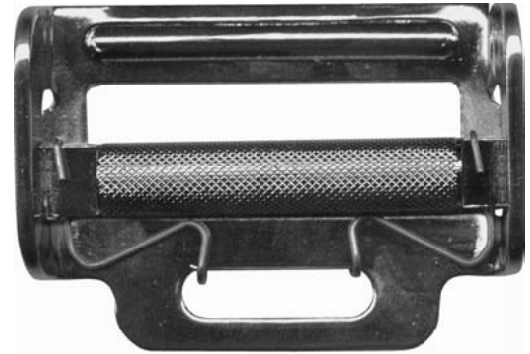
AL14-S Roller Adjuster with Spring Tensioner 2" slot alloy steel, chrome plated 3,000 lb
