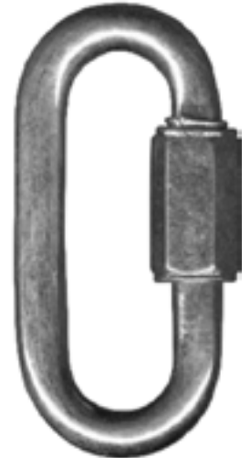
QL53 9/32" steel wire, zinc plated 2 9/16" length 5/16" gate opening
