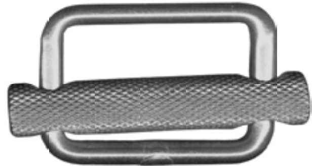
SL2517 Slide Adjuster 1 3/4" with knurled roller bar .250" 304 stainless steel wire SPECIAL ORDER
