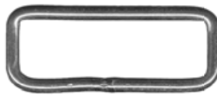
LP3700 Welded Loop 2" x 9/16" .1746" stainless steel wire SPECIAL ORDER
