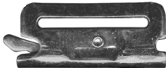
ET-A/200 E-Track Fitting - Spring Actuated 2" web slot steel, zinc plated 4,500 lb breaking strength SPECIAL ORDER
