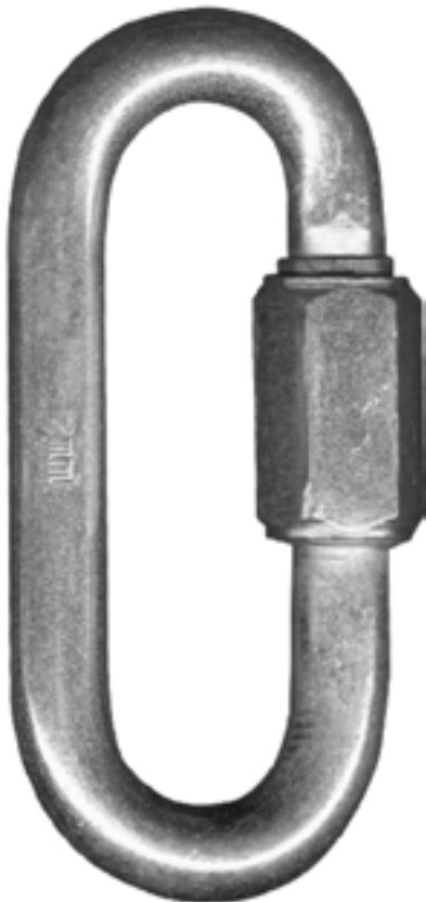
QL57 1/2" steel wire, zinc plated 4 3/16" length 9/16" gate opening
