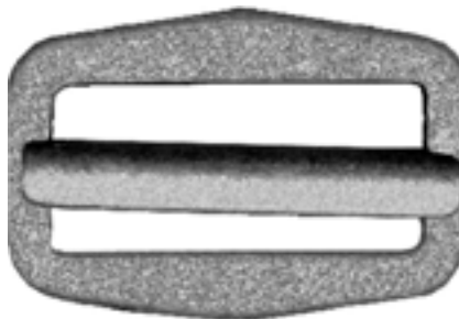
RH11 channel adjuster bar 1 3/4" steel, cadmium plated Certifies to PS70101 500 lb. proof load
