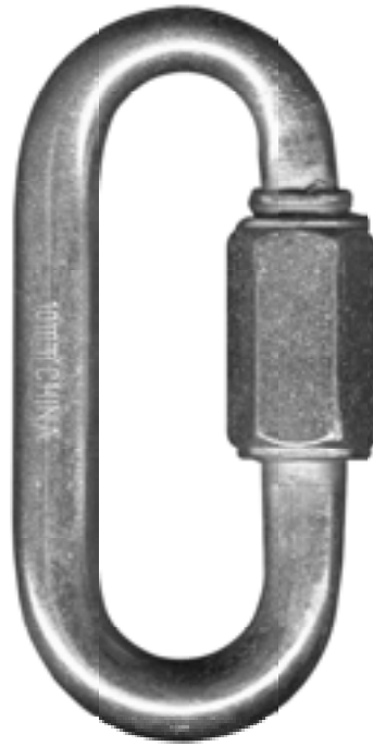
QL56 13/32" steel wire, zinc plated 3 1/2" length 1/2" gate opening
