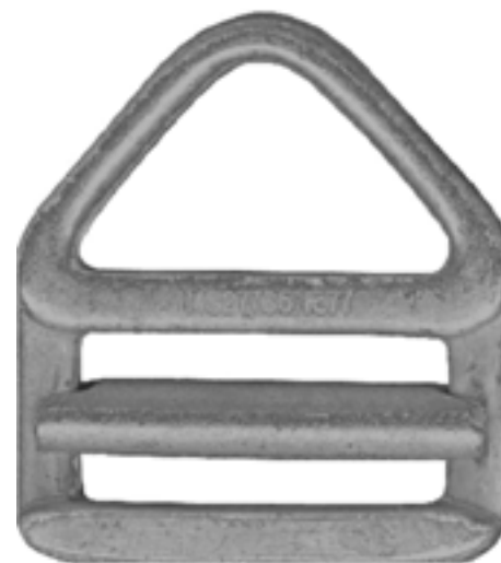
RH18 "Quick Fit Adjuster" 1 3/4" slot forged steel, cadmium plated 2,500 lb. proof load Certifies to PS27765
