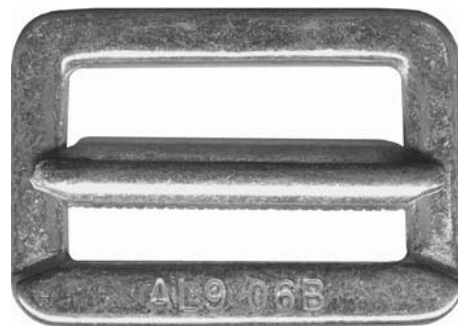
AL9 knurled adjuster bar 1 3/4" x 1" forged steel, zinc plated 5,000 lb Commercial version of PS22040
