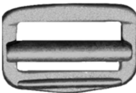
RH8 channel adjuster bar 1 3/4" x 3/4" forged steel, cadmium plated 2,500 lb proof load Certifies to PS22019 SPECIAL ORDER
