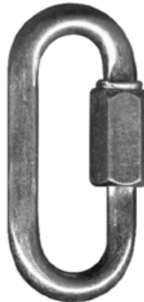
QL55 3/8" steel wire, zinc plated 3 5/16" length 1/2" gate opening Use QL69 for Stainless Steel
