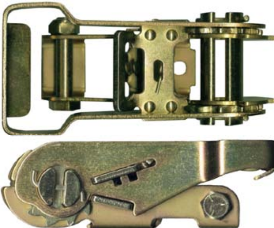
RAT/100-1200 Ratchet 1" steel, yellow chromate plated 1,200 lb
