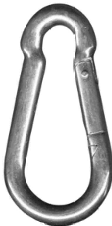
SPC60 13/32" steel wire, zinc plated 3 7/8" length 9/16" gate opening Use SP74 for Stainless Steel
