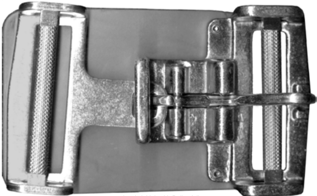
Latch & Link with Roller Adjusters with leather pad RH7116 3" forged steel, zinc plated 3,000 lb
