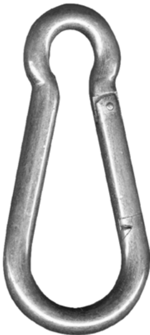
SP58 1/2" steel wire, zinc plated 5 1/2" length 3/4" gate opening
