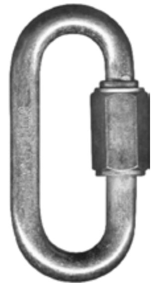
QL54 5/16" steel wire, zinc plated 3" length 3/8" gate opening Use QL68 for Stainless Steel
