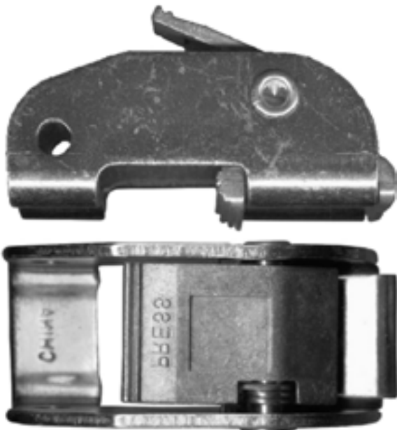
CAM/100-1800 1" steel, yellow chromate plated 1,800 lb
