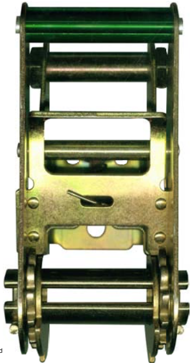
RAT/200-10000 Ratchet 2" steel, yellow chromate plated 10,000 lb
