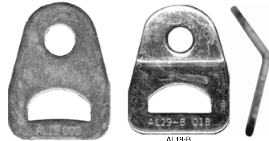
AL19 Bolt-In End Fitting 1" x 1/2" slot, 1/2" hole alloy steel, yellow chromate plated 3,000 lb
