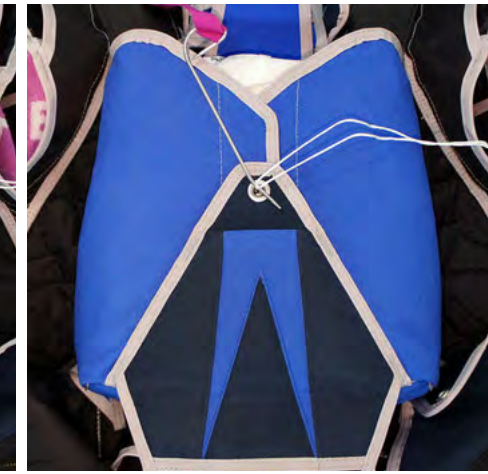
24. Close the bottom flap (#5).
