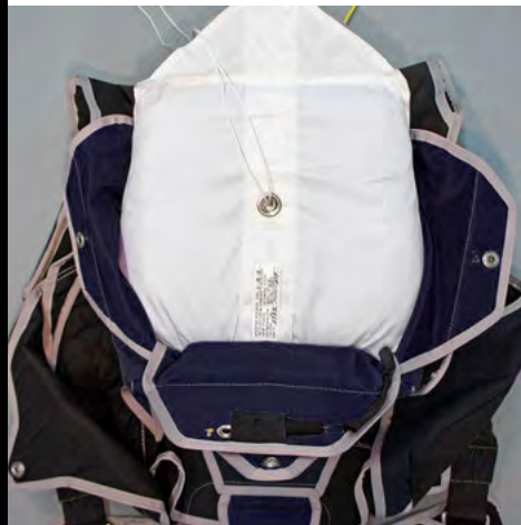
12. Rotate Freebag into reserve container filling lower corners of reserve container.
