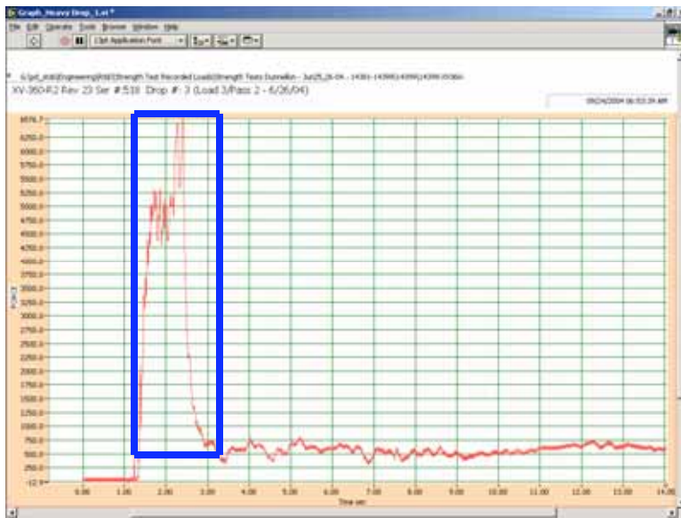
(Top) Graph of parachute deployment including approximately 10 secs of flight. The box highlights the parachute deployment.
