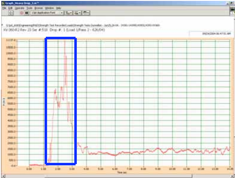
(Top) Graph of parachute deployment including approximately 10 secs of flight. The box highlights the parachute deployment. Exploded view shown below.
