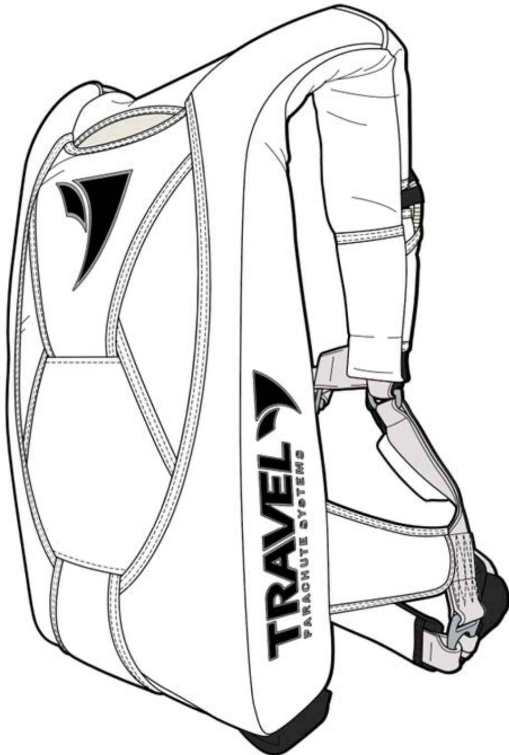
PIC – 6 – Drawing Side View
